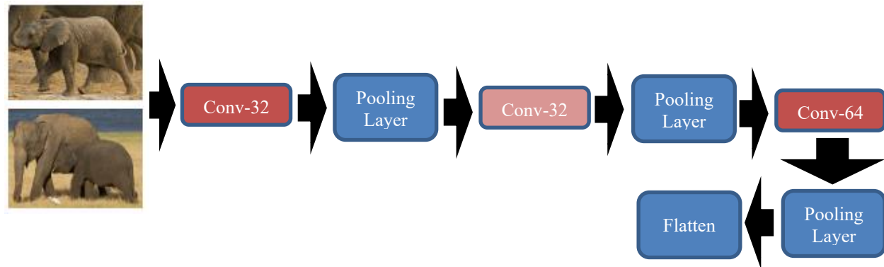
Fig 2. VGG-16 Architecture
